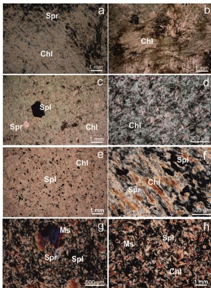
Fig. 6: Micro-hotomicrographs in plane-polarized light (PPL) and crossed-polars (XPL) of some of the studied samples showing the main features described in the text.: a) sample 08, PPL; b) sample 13, PPL; c) sample 22, PPL; d) sample 23, PPL; e) sample 24, PPL; f), sample 26, XPL; g) sample 21, XPL; h) sample 24, XPL.
