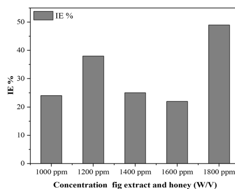
Figure 3. Bar chart illustrating the calculated percentage inhibition efficiency of Sidr honey and fig sap in the presence of a 0.5 M sodium chloride solution.
