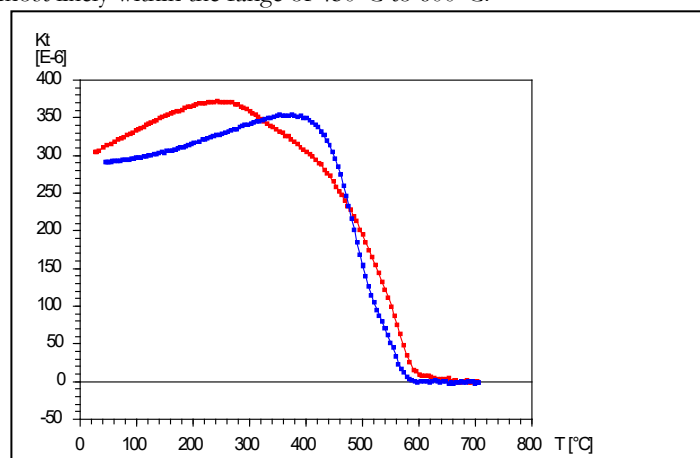
Figure 3. The D.G5 sample exhibits high susceptibility and is irreversible, containing pyrrhotite and magnetite minerals.
